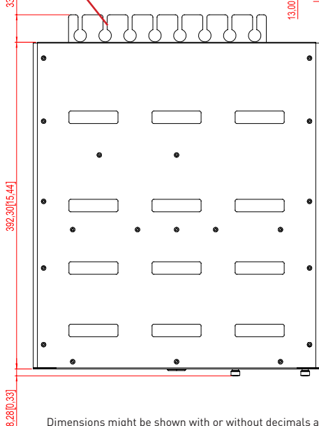
Cable/Retainer Kit TOP VIEW
